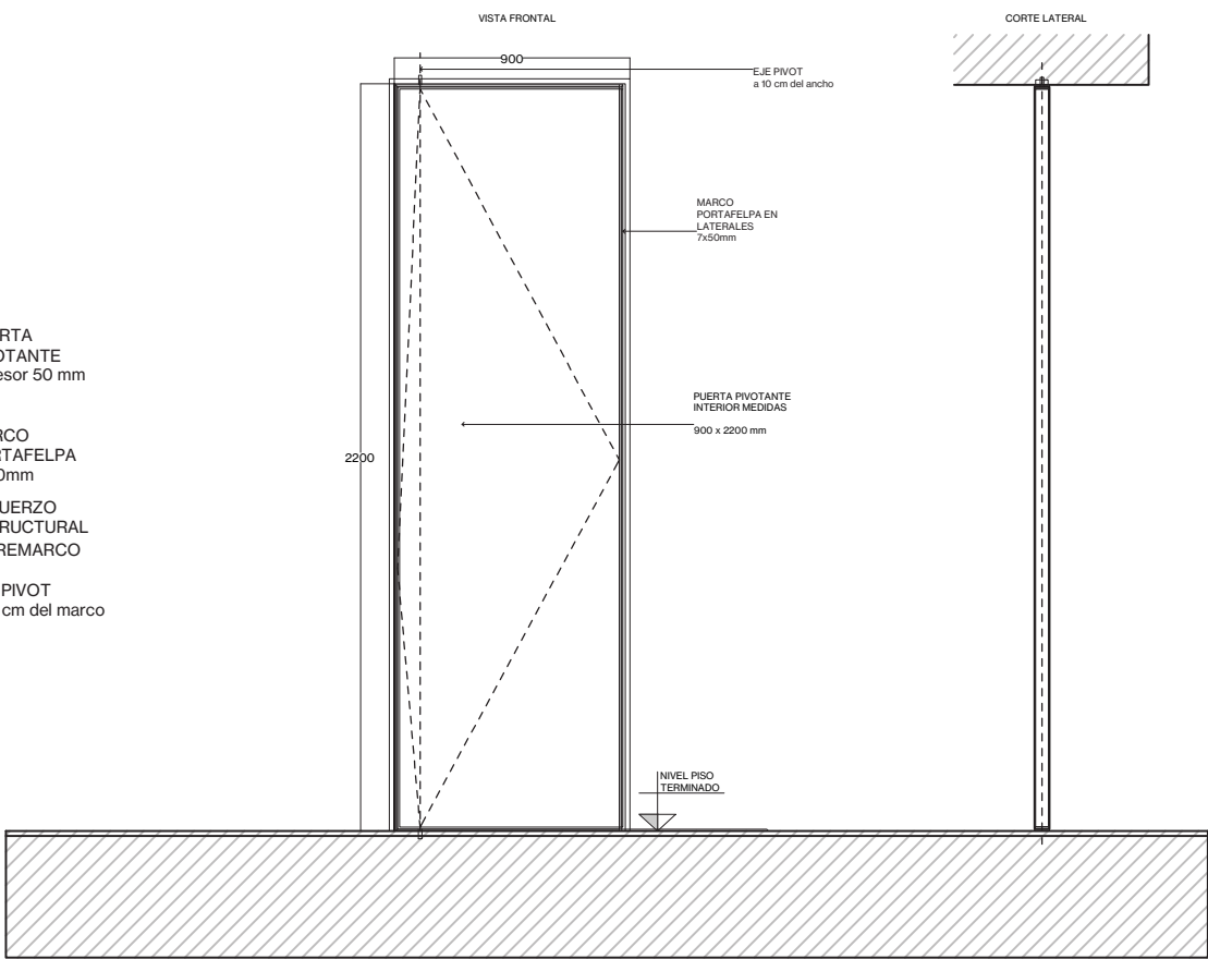
Vista Frontal Exterior
