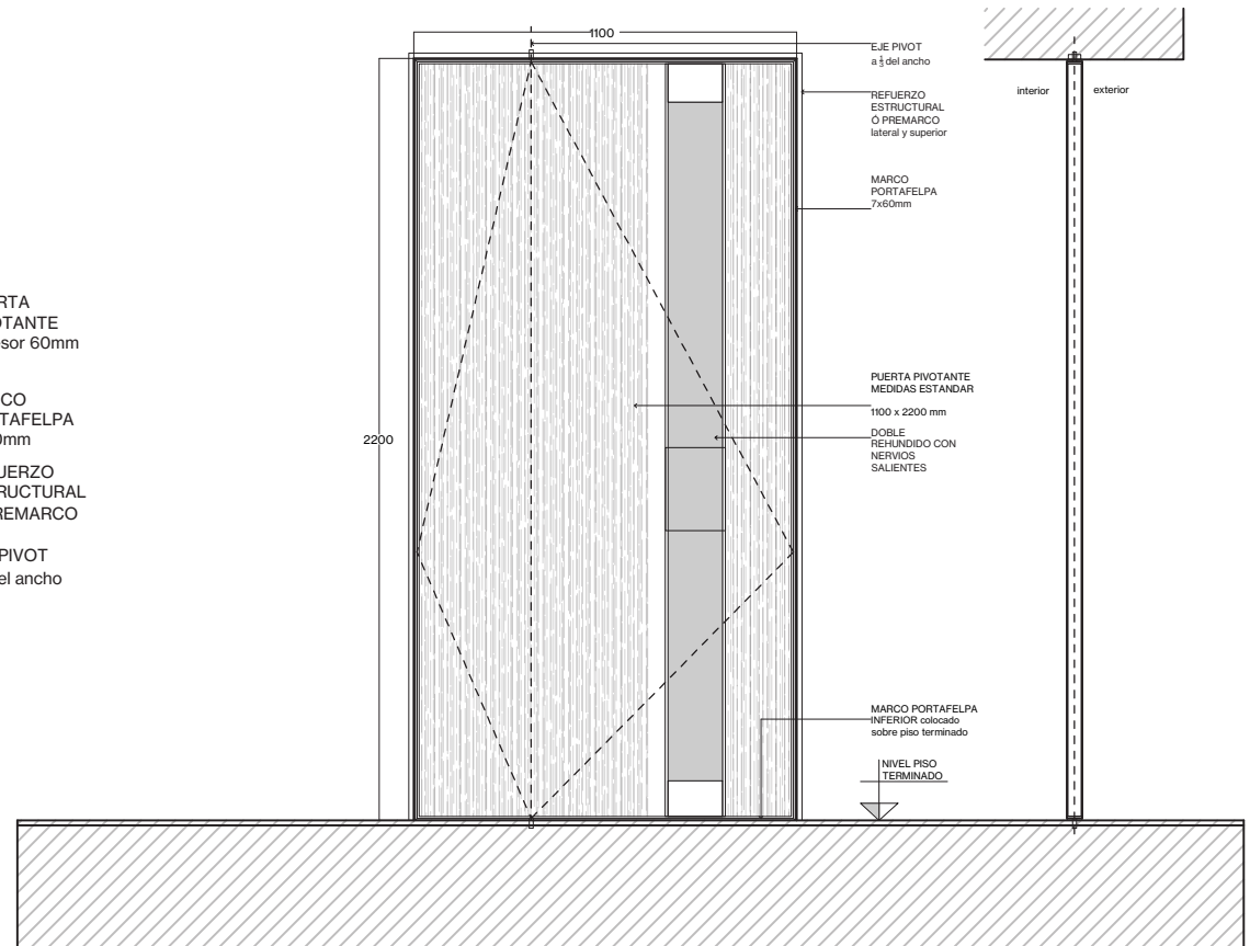
Vista Frontal Exterior
