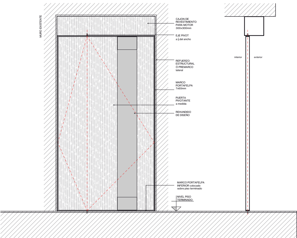
Vista Frontal Exterior
