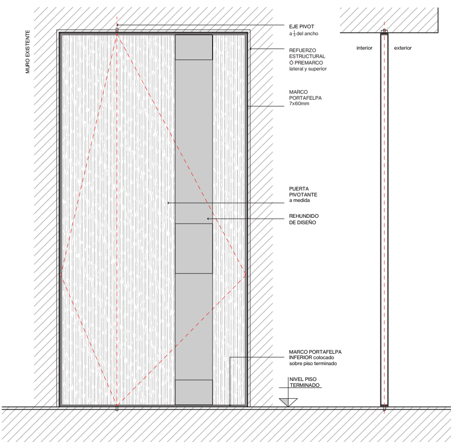
Vista Frontal Exterior
